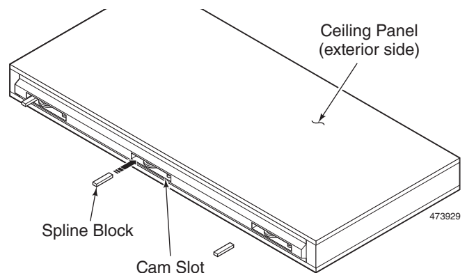
Figure 24. Spline Blocks
