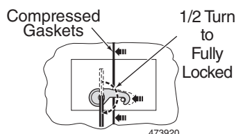
Figure 4. Locked Position
