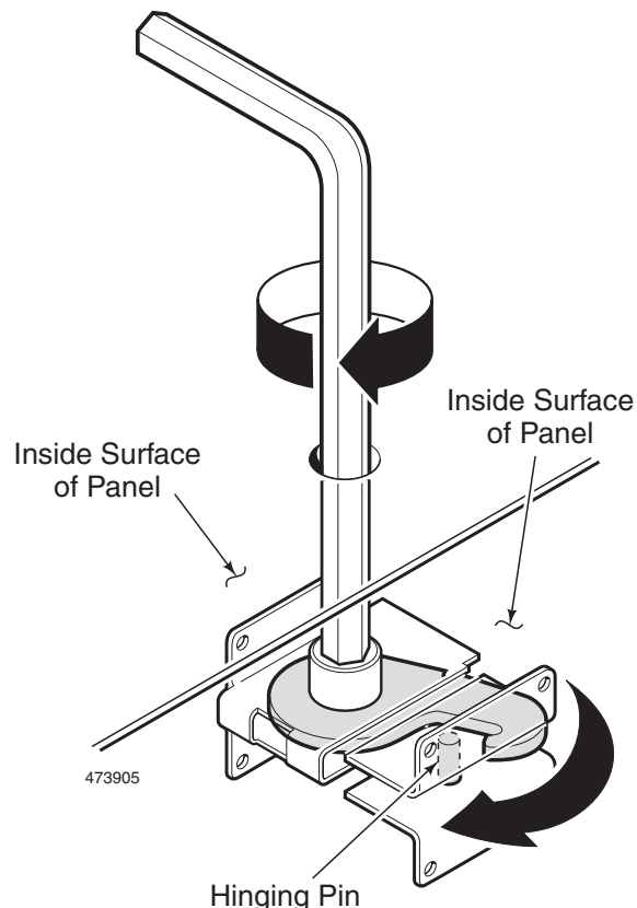
Figure 5. Cam Lock Fastener
