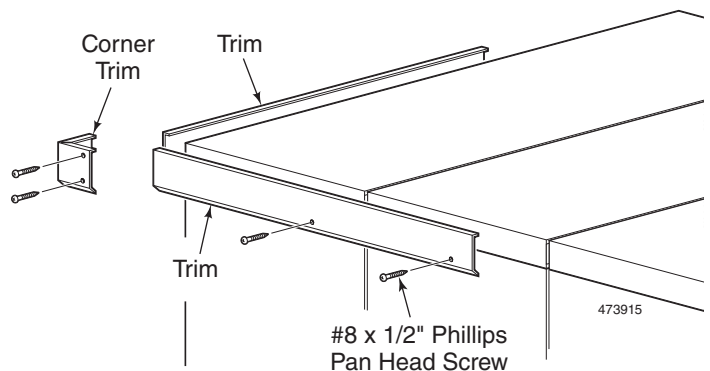
Figure 32. Ceiling Trim
