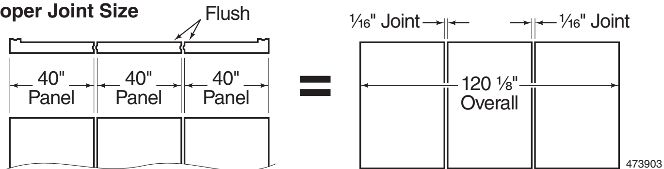
Figure 6. Assembling Panels
