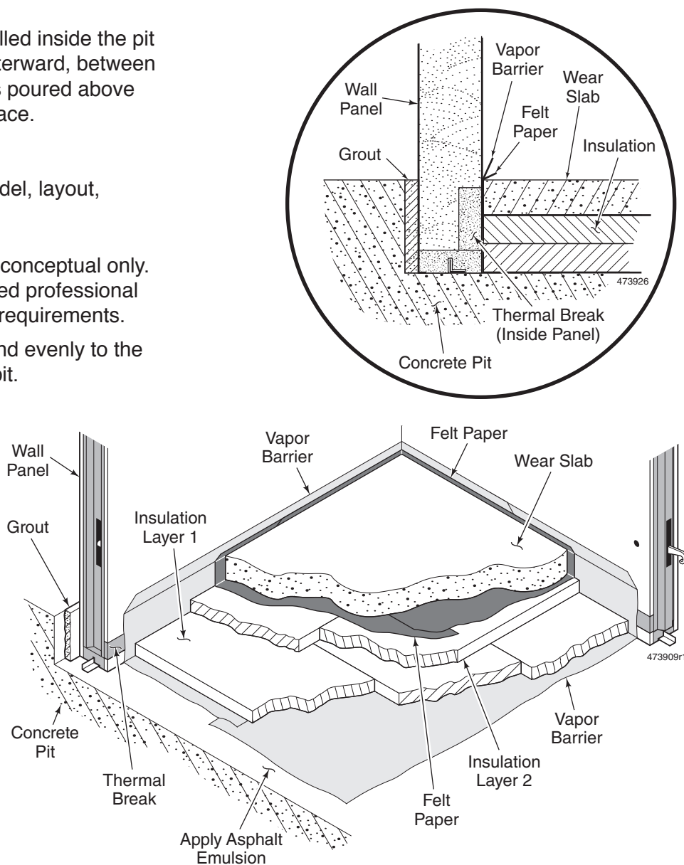
Figure 14. Insulated Pit with Wall Panels Below Grade
