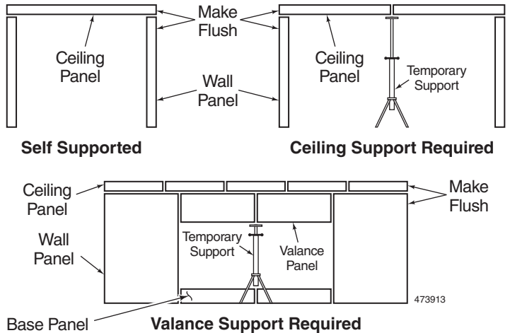
Figure 21. Support
