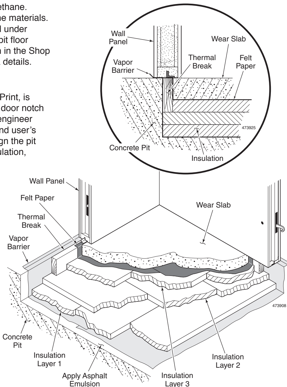
Figure 13. Insulated Pit with Wall Panels Above Grade
