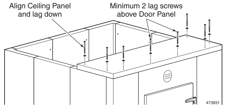
Figure 22. First Panel
