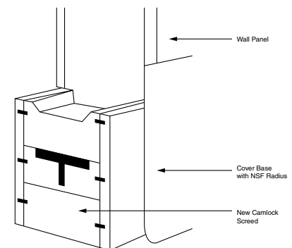
Figure 19. Floor Spline
