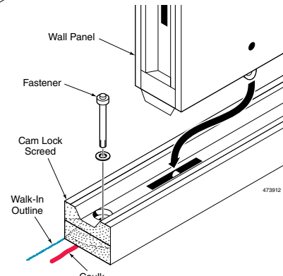
Figure 18. Cam Lock Screed
