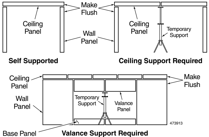
Figure 23. Support
