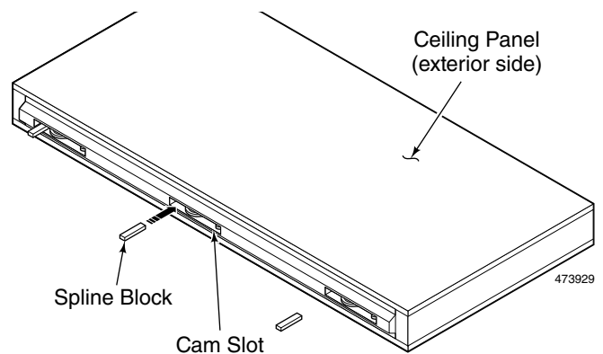
Figure 26. Spline Blocks
